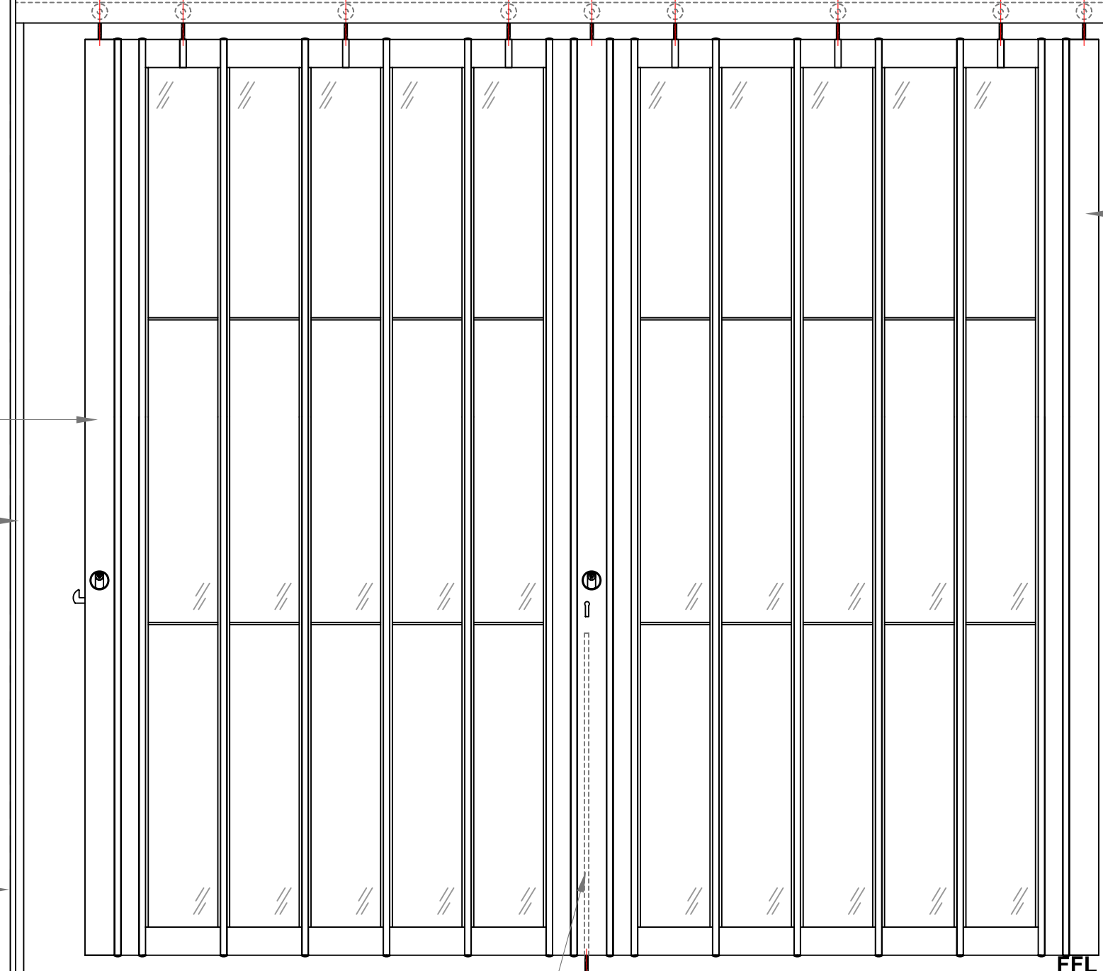
FRONT ELEVATION 1:10
