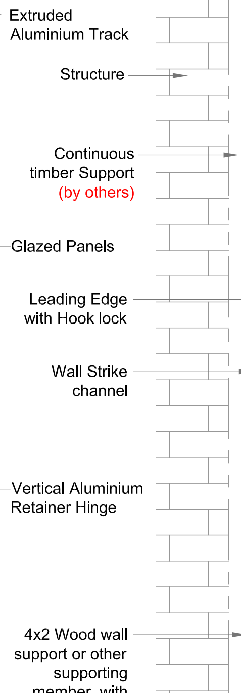
FRONT ELEVATION 1:10
